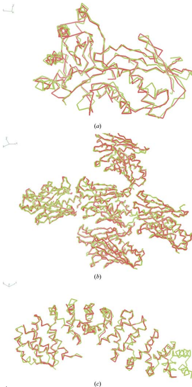
Figure 4 Backbone diagrams of chain tracings. (a) Mevalonate kinase (PDB entry 1kkh; Yang et al. , 2002). (b) Structural genomics target 1038B (PDB entry 1lqj; Choi et al. , 2003). (c) Armadillo repeat region of murine \beta -catenin (PDB entry 3bct; Huber et al. , 1997). Red tracings are from the present method; green tracings are from the deposited structures. These figures were created with Coot (Emsley & Cowtan, 2004).
